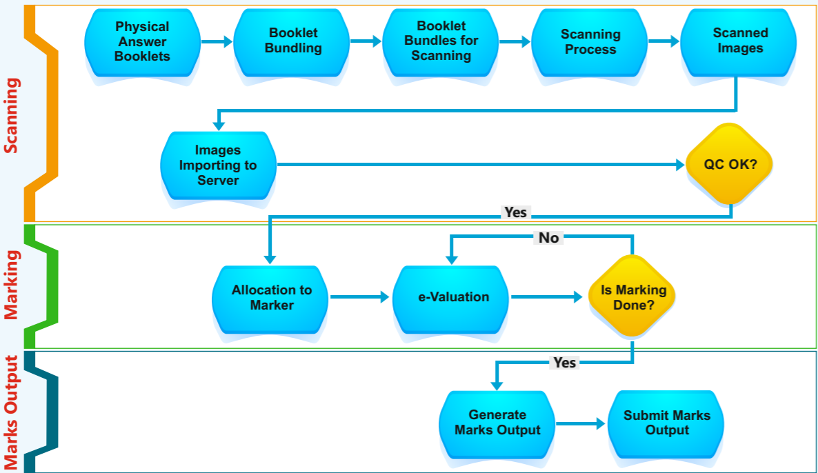
Workflow of the Answer-Book Digitization and Onscreen Marking
